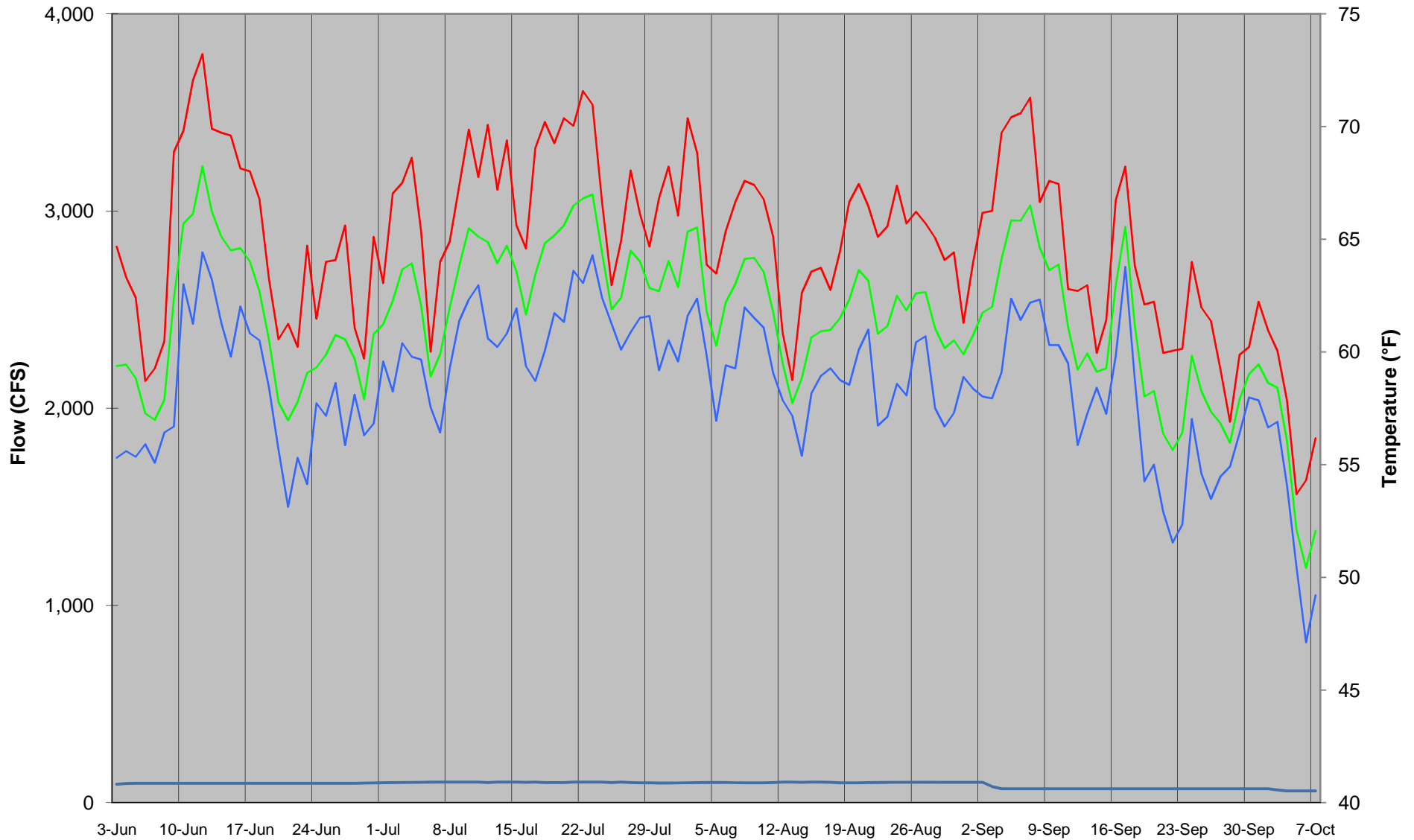
Appendix 1W. Summer daily average, maximum, and minimum water temperature profiles on the Neversink at Ranch Rd bridge, along with daily average flows at Neversink, 2008.
