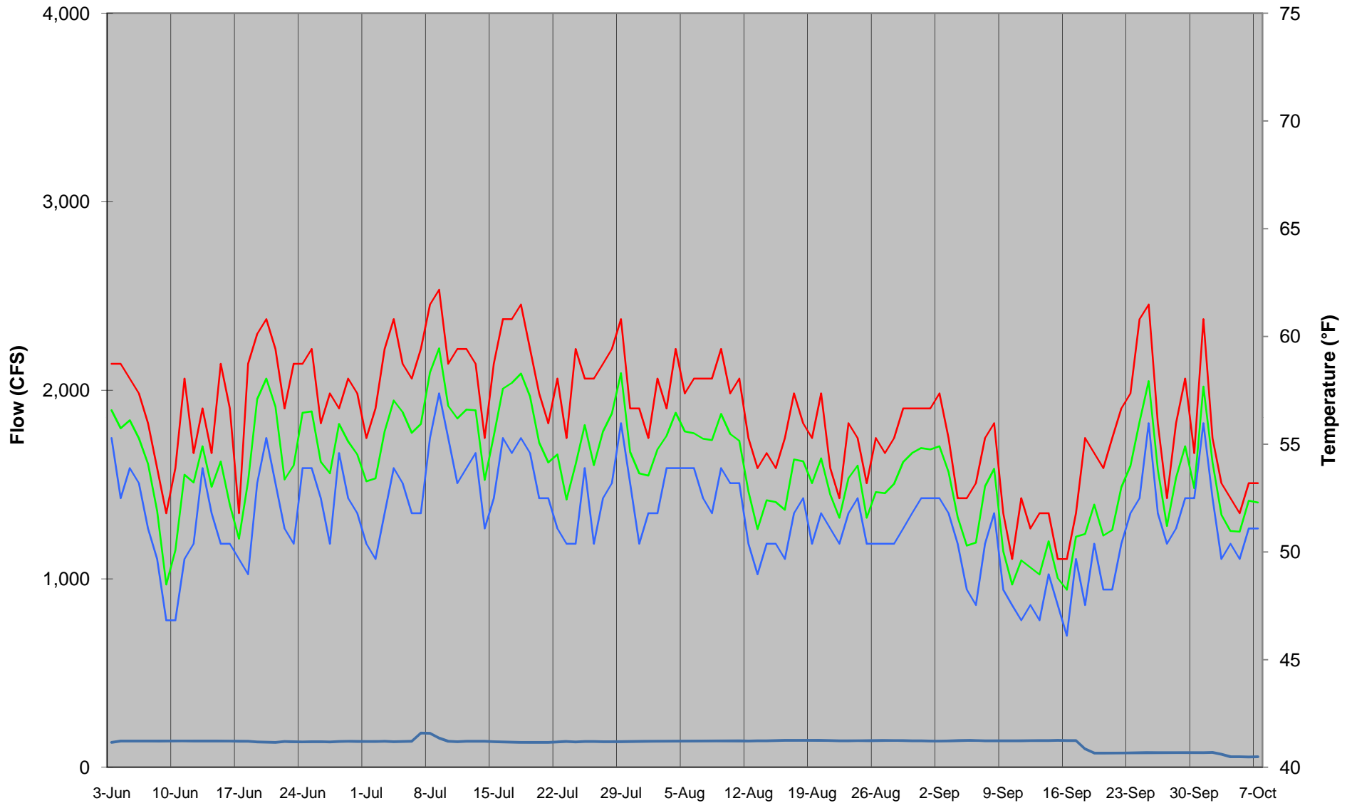
Appendix 3K. Summer daily average, maximum, and minimum water temperature profiles on the East Branch at Shinhopple, along with daily average flows at Downsville, 2010.
