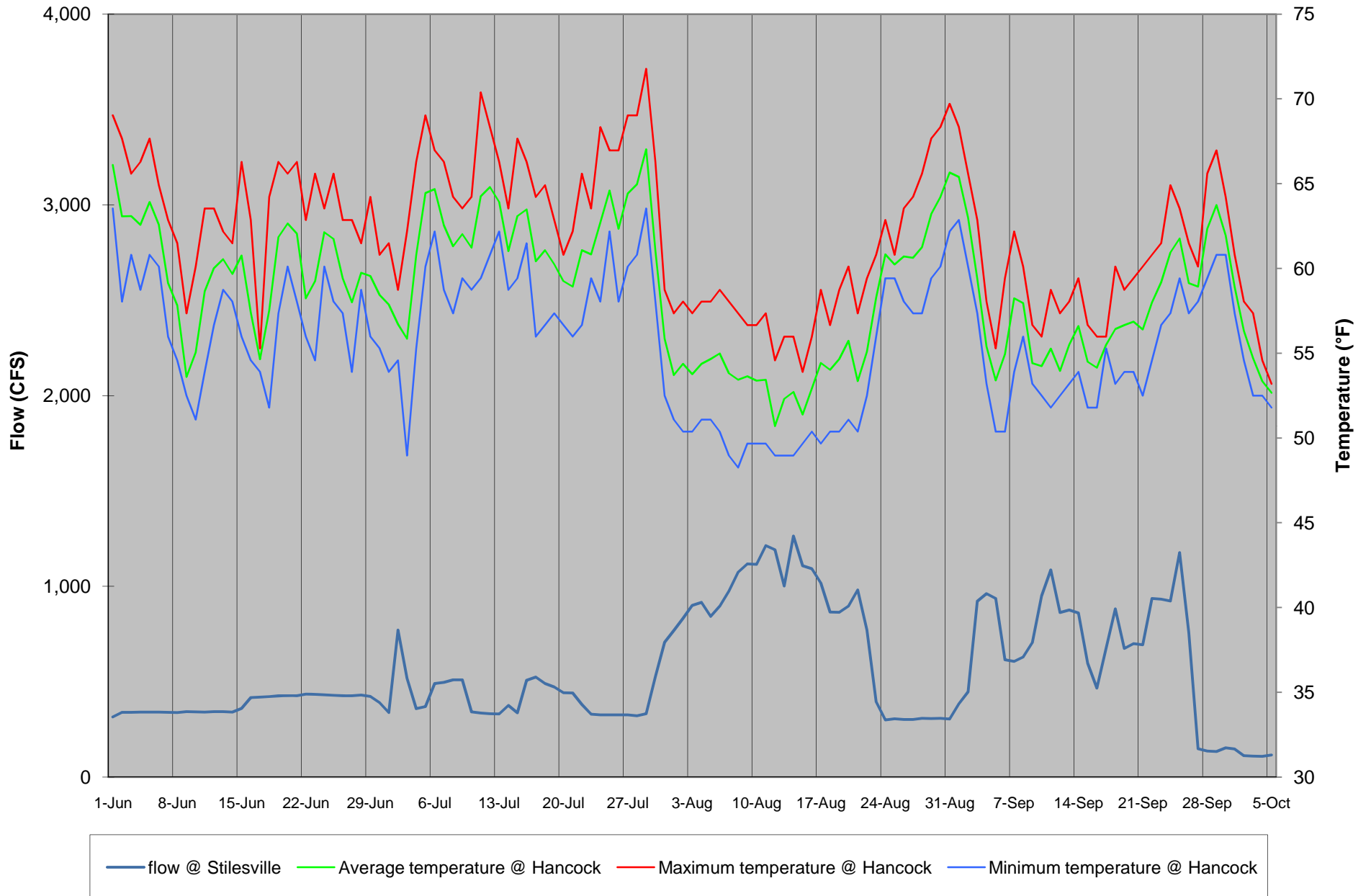
Appendix 3G. Summer daily average, maximum, and minimum water temperature profiles on the West Branch at Hancock, along with daily average flows at Stilesville, 2010.
