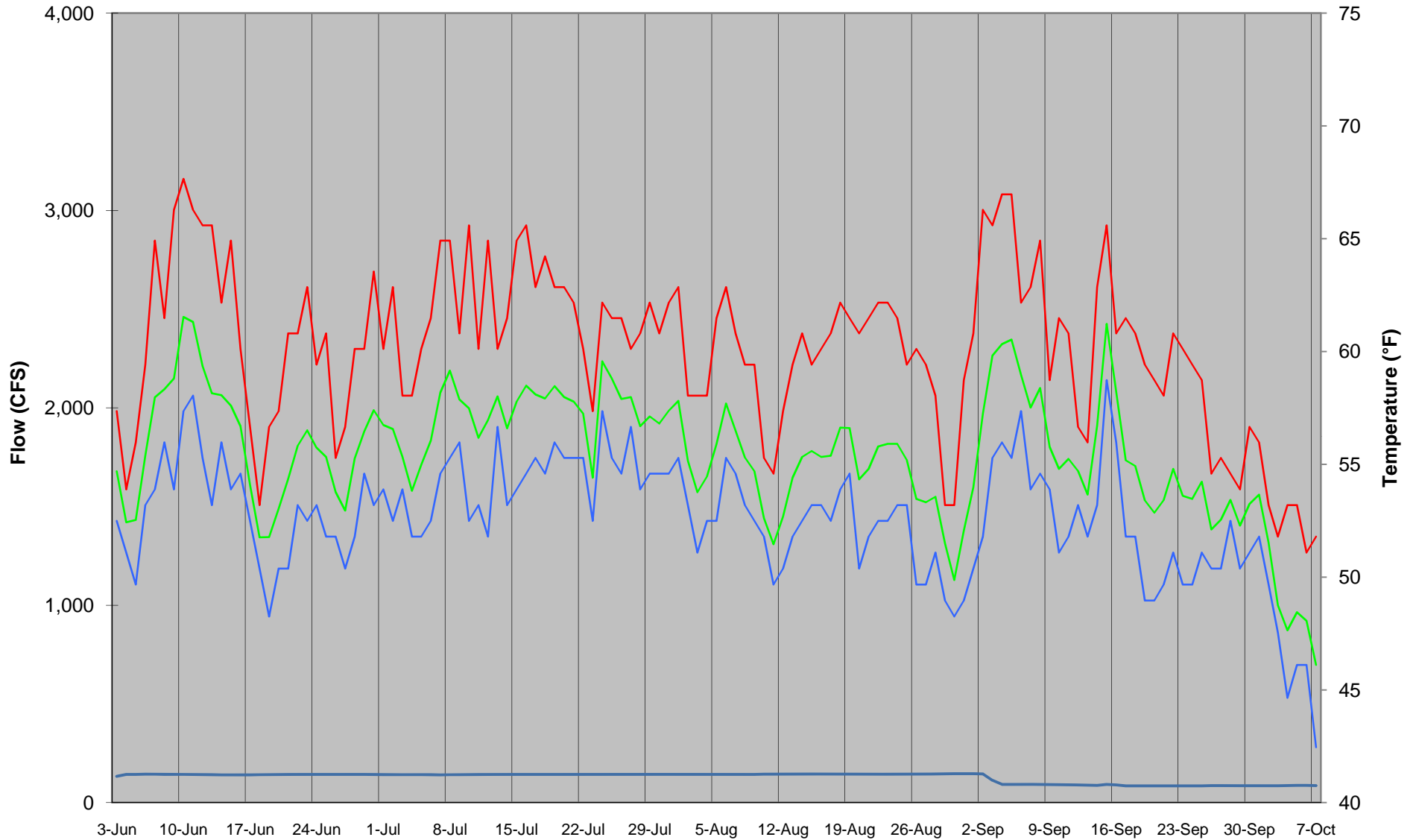
Appendix 1M. Summer daily average, maximum, and minimum water temperature profiles on the East Branch at Terry's Campsite, along with daily average flows at Downsville, 2008.
