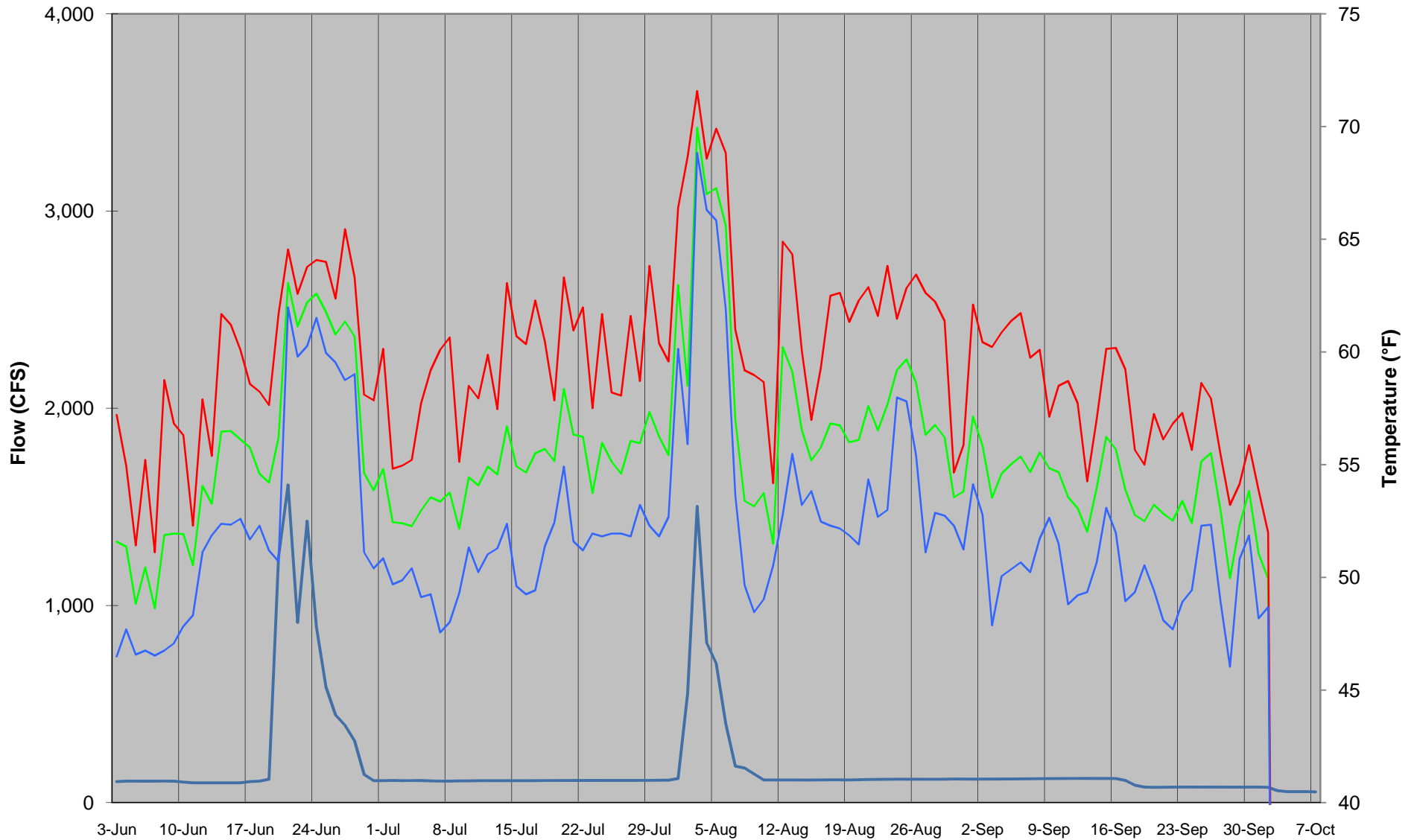
Appendix 2U. Summer daily average, maximum, and minimum water temperature profiles on the Neversink at Woodbourne, along with daily average flows at Neversink, 2009.
