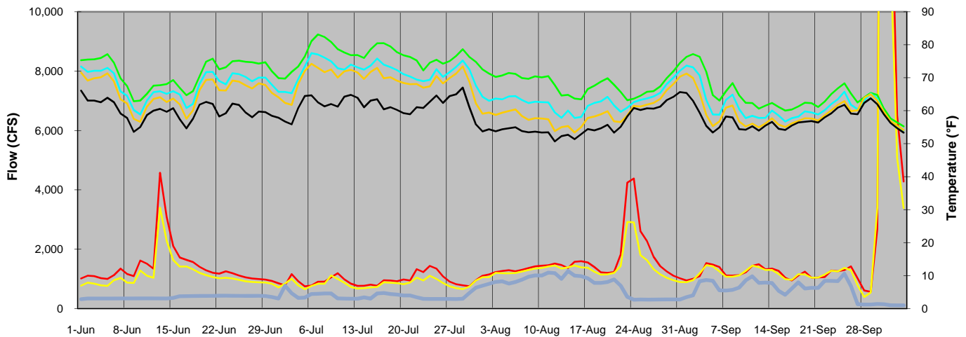
Figure 8: Longitudinal summer daily average temperature profile on the West Branch at Hancock and Leonards Abe Lord, and Callicoon on the Delaware River along with the daily average flows at Stilesville on the West Branch and Lordville and Callicoon on the Delaware River, 2008-2010.
