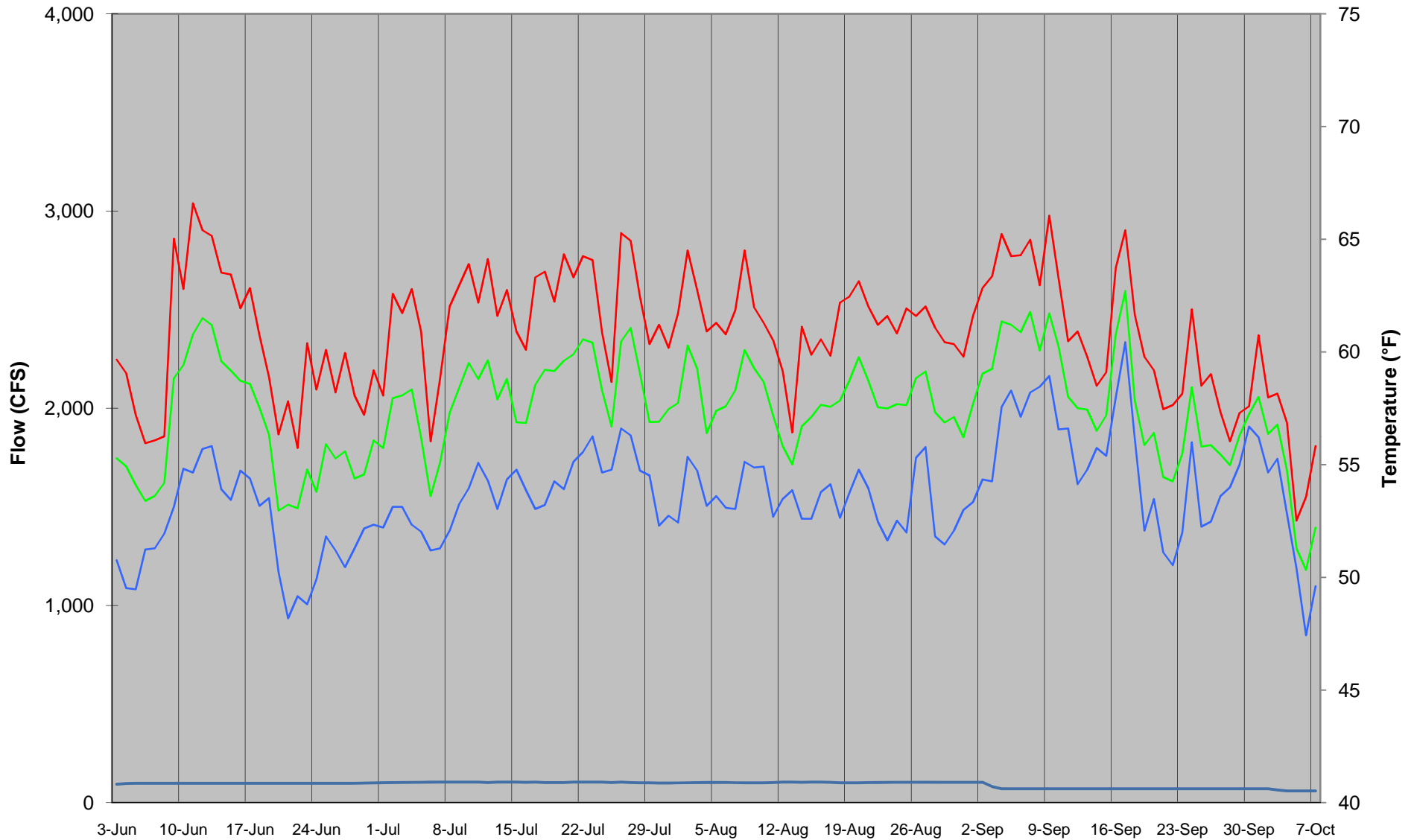
Appendix 1V. Summer daily average, maximum, and minimum water temperature profiles on the Neversink just above Fallsburg, along with daily average flows at Neversink, 2008.
