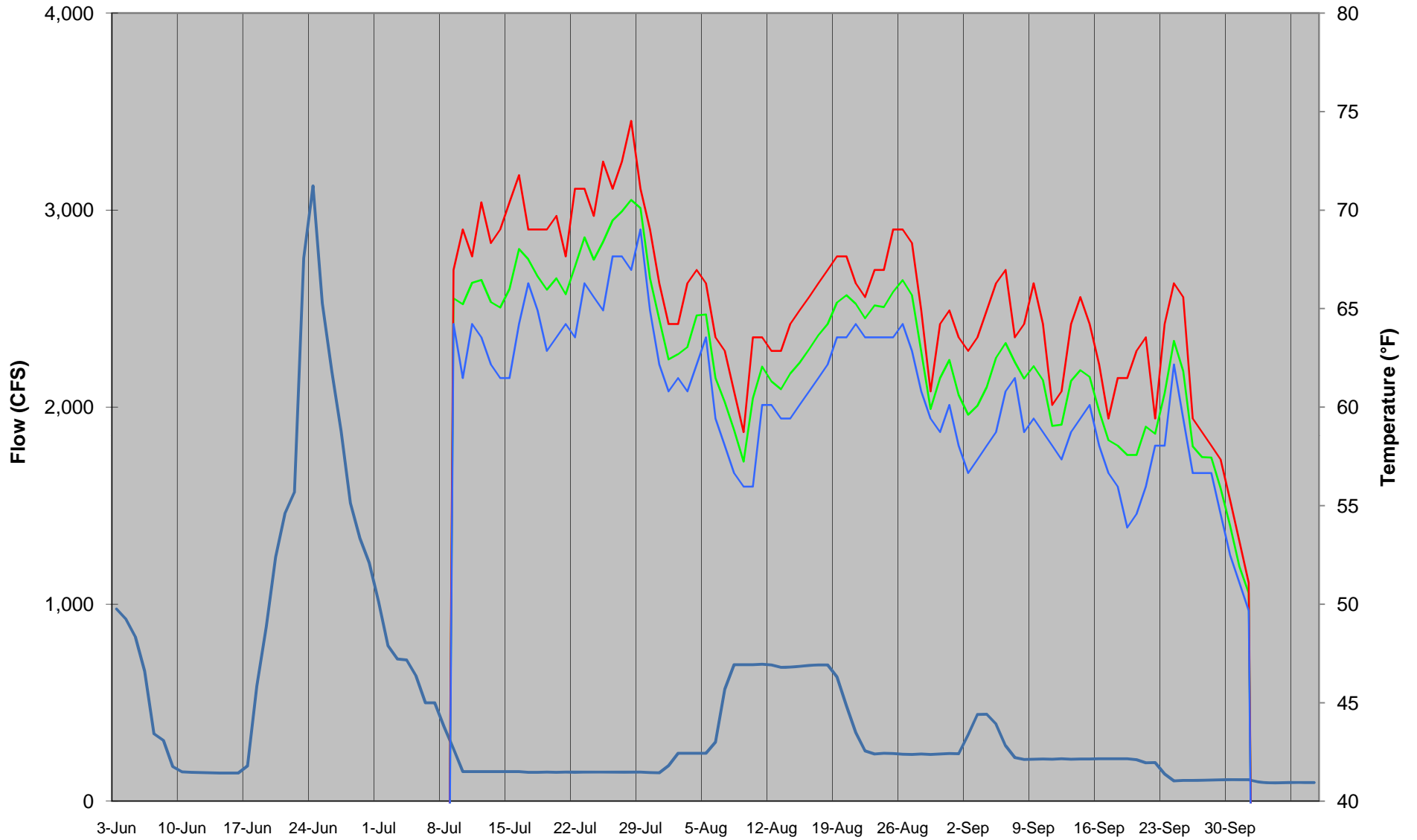
Appendix 2S. Summer daily average, maximum, and minimum water temperature profiles on the East Branch at Hancock, along with daily average flows at Downsville, 2009.
