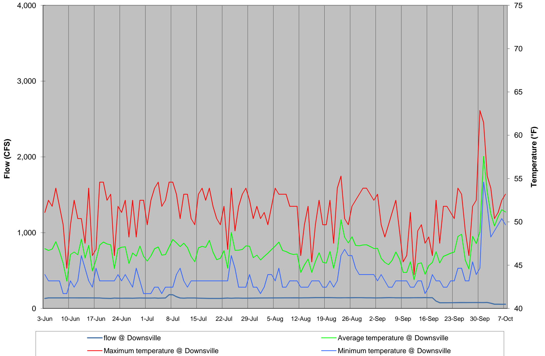
Appendix 3J. Summer daily average, maximum, and minimum water temperature profiles on the East Branch at Downsville, along with daily average flows at Downsville, 2010.
