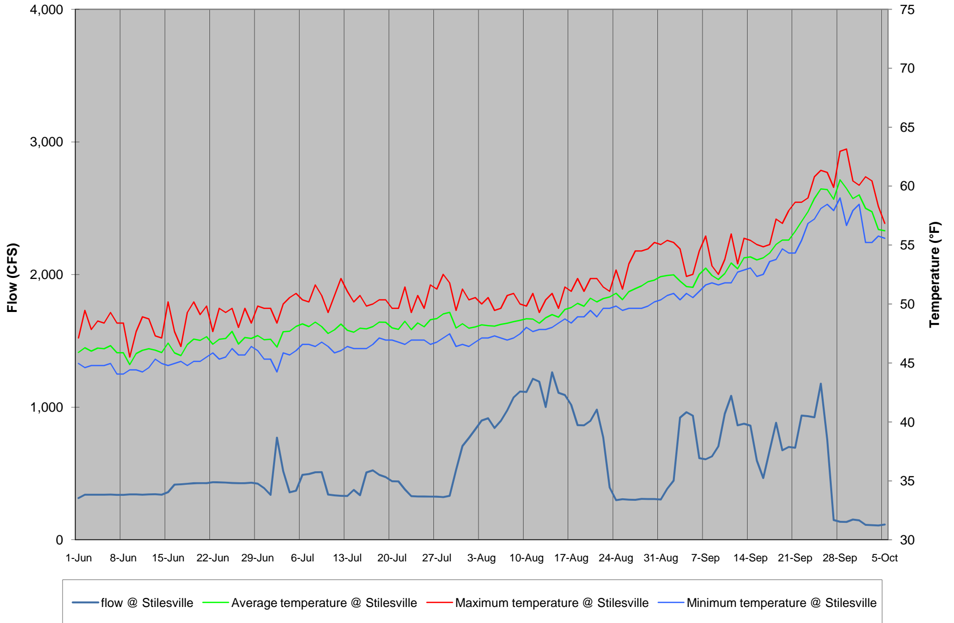
Appendix 3A. Summer daily average, maximum, and minimum water temperature profiles from the USGS gage on the West Branch at Stilesville, along with daily average flows at Stilesville, 2010.
