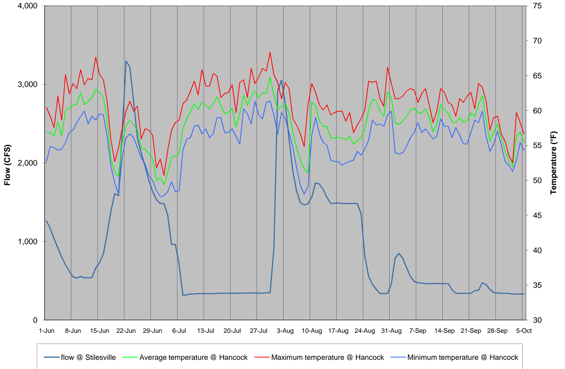
Appendix 2I. Summer daily average, maximum, and minimum water temperature profiles from the USGS gage on the West Branch at Hancock, along with daily average flows at Stilesville, 2009.
