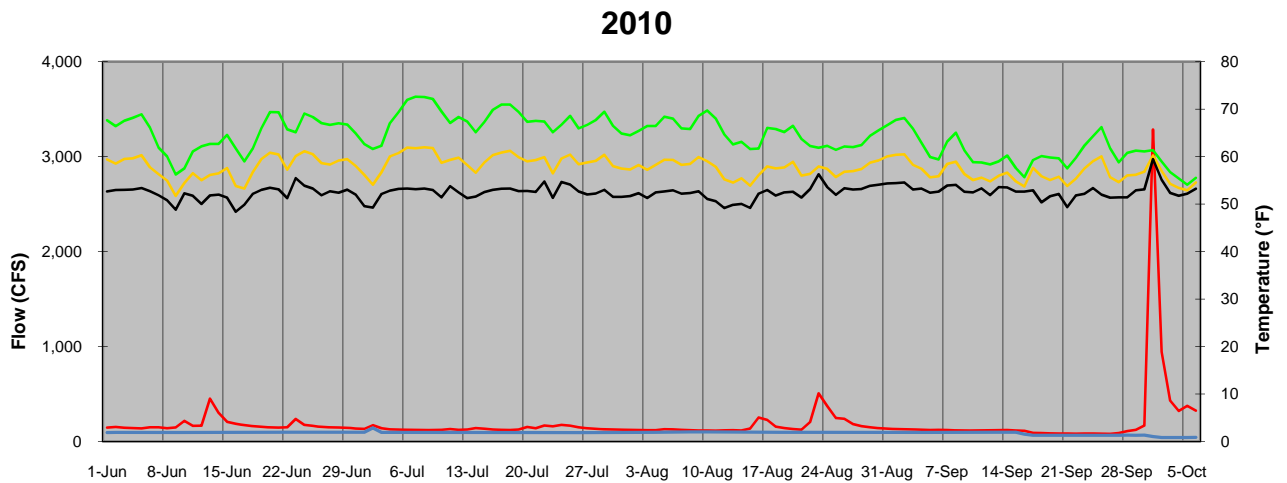
Figure 6: Longitudinal summer average water temperature profile on the Neversink River at Bridgeville, Fallsburg, and Hasbrouck along with daily average flows at Bridgeville and Neversink just below the dam, 2008-10.
