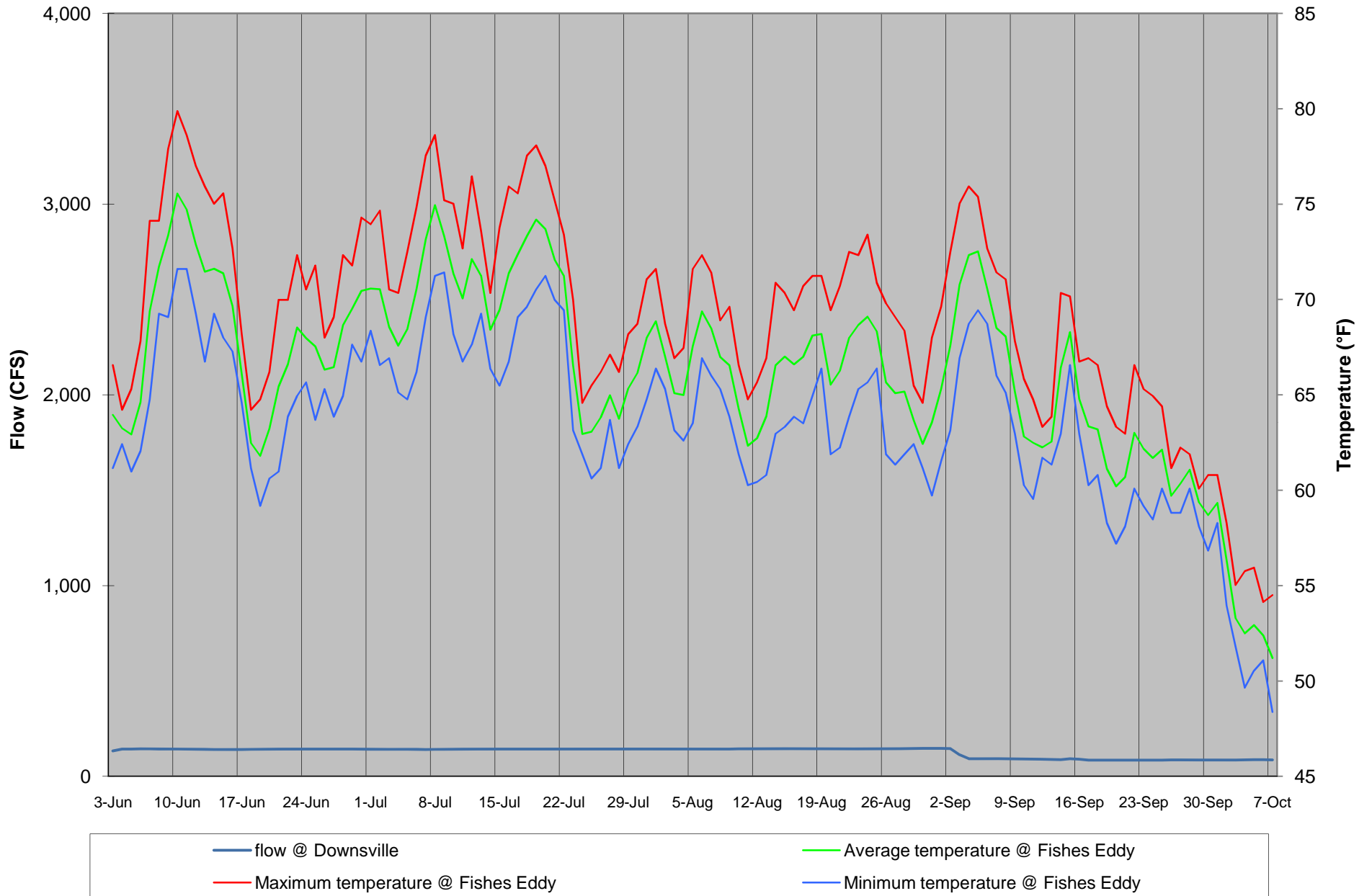
Appendix 1R. Summer daily average, maximum, and minimum water temperature profiles from the USGS gage on the East Branch at Fishes Eddy, along with daily average flows at Downsville, 2008.
