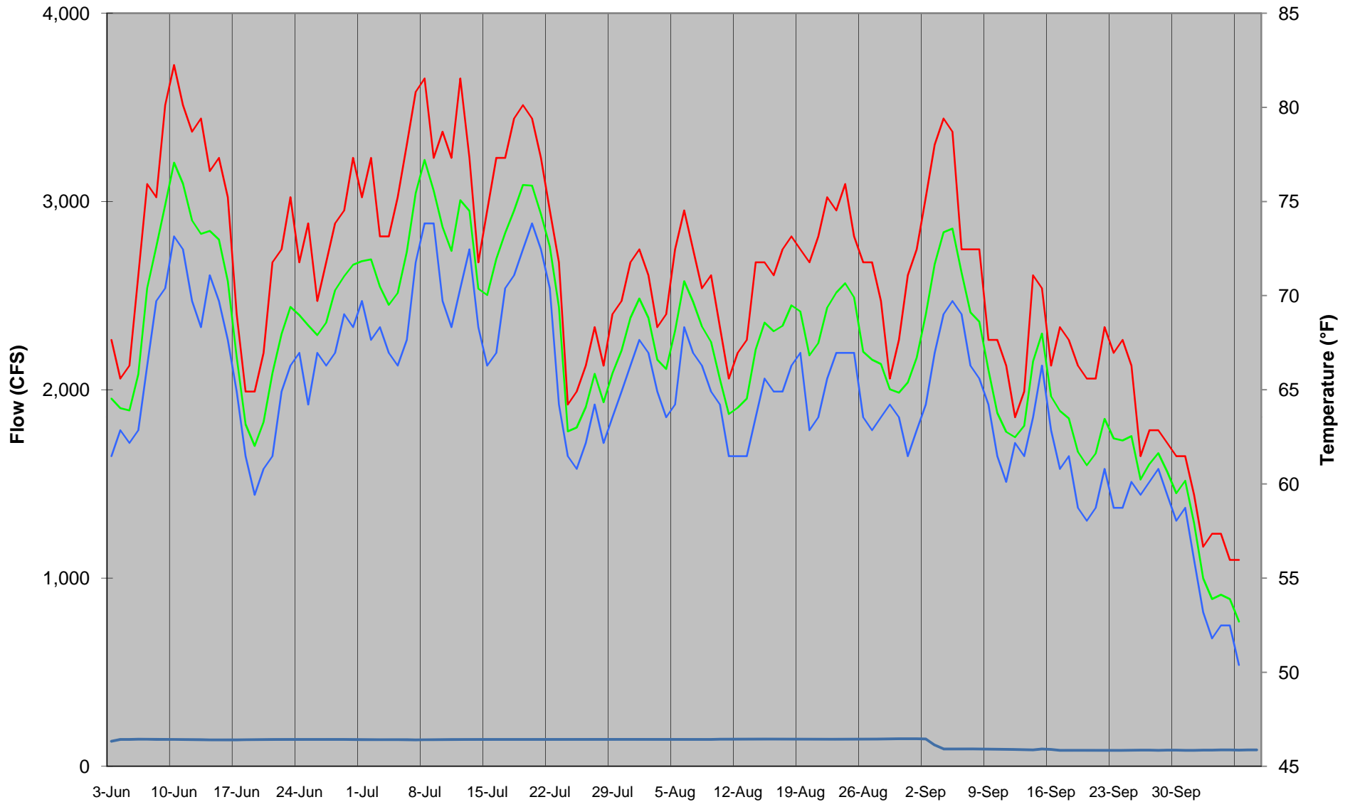
Appendix 1S. Summer daily average, maximum, and minimum water temperature profiles on the East Branch at Hancock, along with daily average flows at Downsville, 2008.
