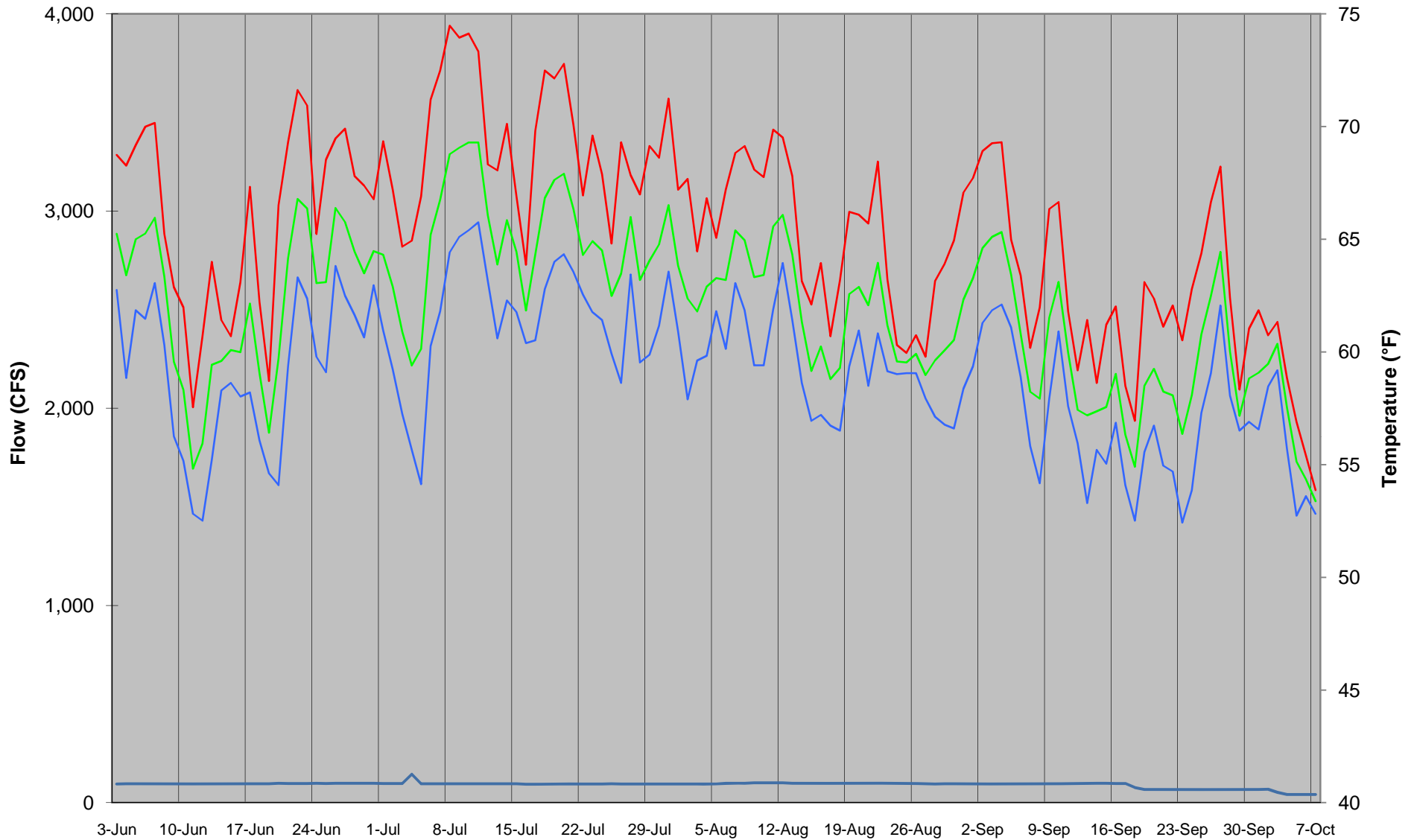
Appendix 3U. Summer daily average, maximum, and minimum water temperature profiles on the Neversink at Ranch Rd bridge, along with daily average flows at Neversink, 2010.
