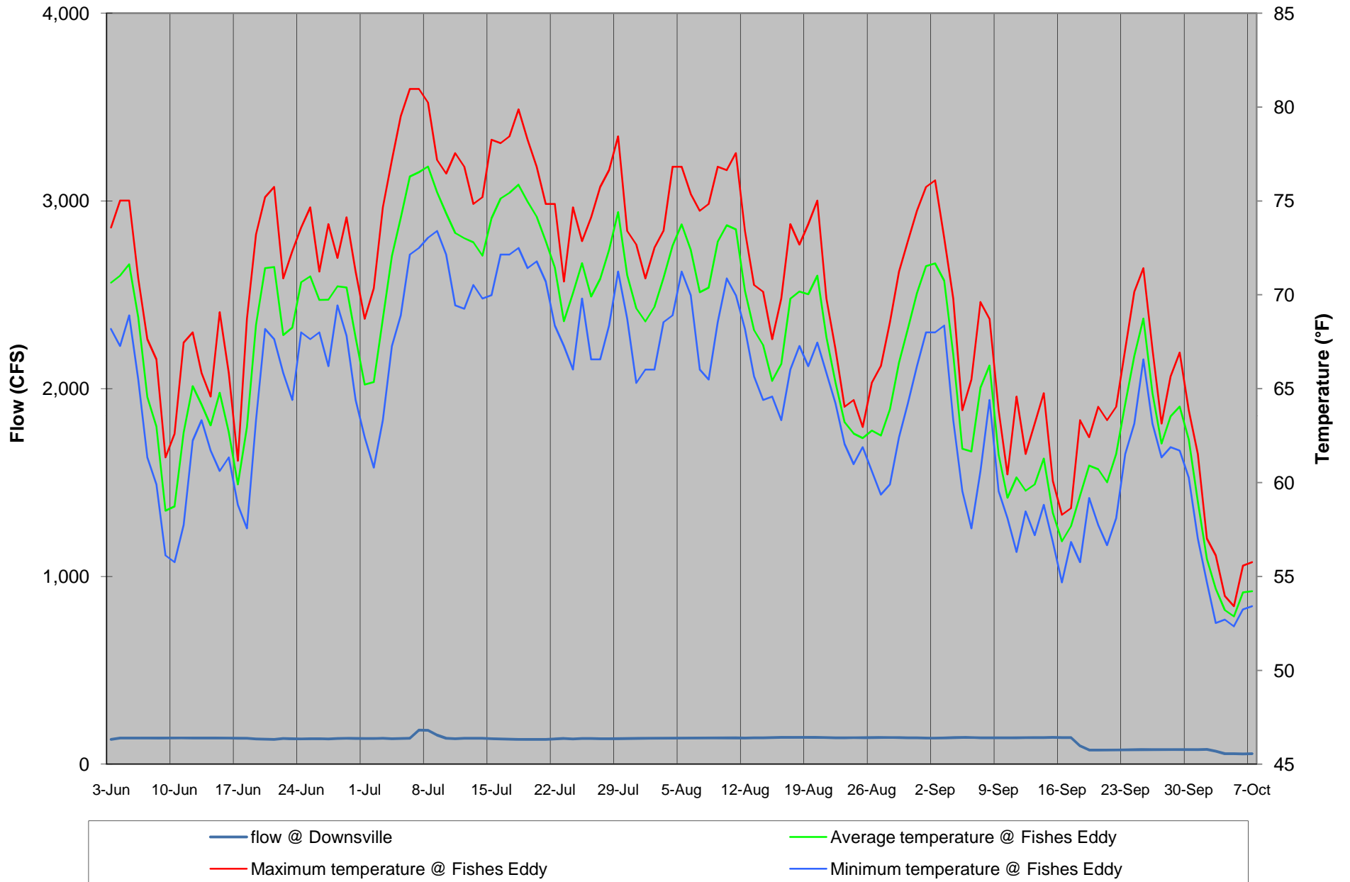
Appendix 3P. Summer daily average, maximum, and minimum water temperature profiles from the USGS gage on the East Branch at Fishes Eddy, along with daily average flows at Downsville, 2010.
