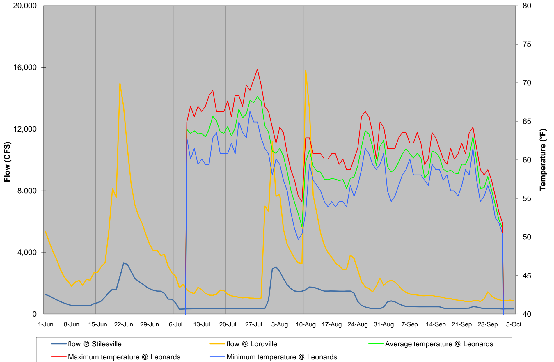
Appendix 2Y. Summer daily average, maximum, and minimum water temperature profiles on the Delaware River at Leonards, along with daily average flows at Stilesville on the West Branch and Lordville, 2009.
