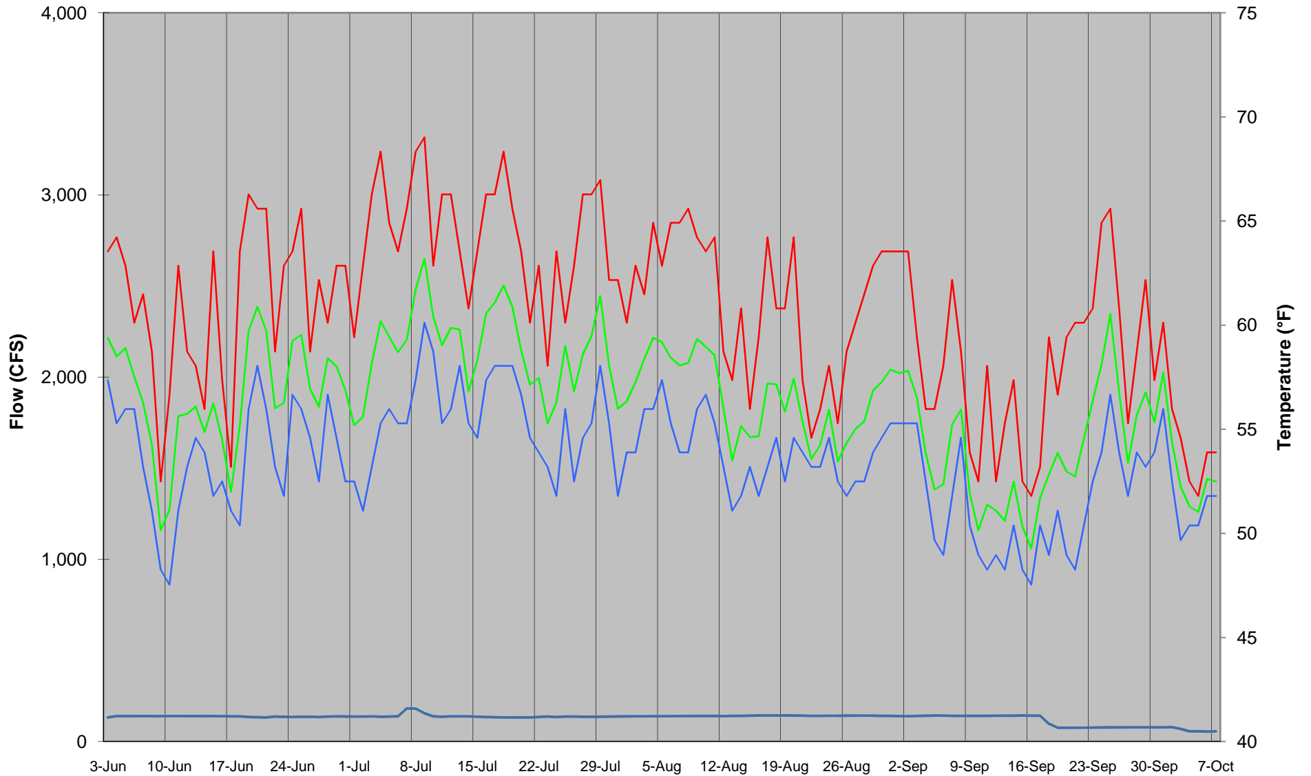
Appendix 3L. Summer daily average, maximum, and minimum water temperature profiles on the East Branch at Terry's Campsite, along with daily average flows at Downsville, 2010.
