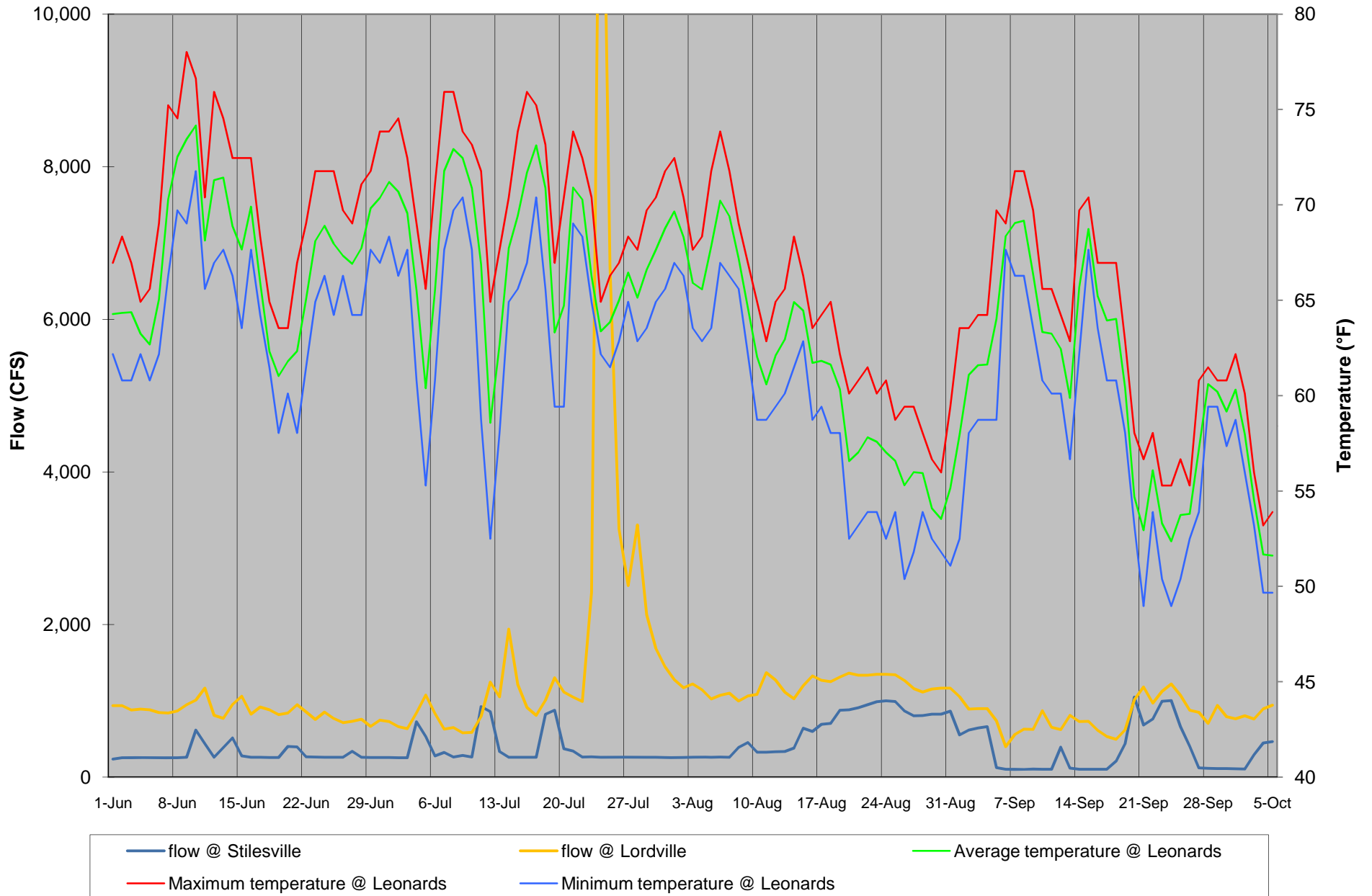
Appendix 1Y. Summer daily average, maximum, and minimum water temperature profiles on the Delaware River at Leonards, along with daily average flows at Stilesville on the West Branch and Lordville, 2008.
