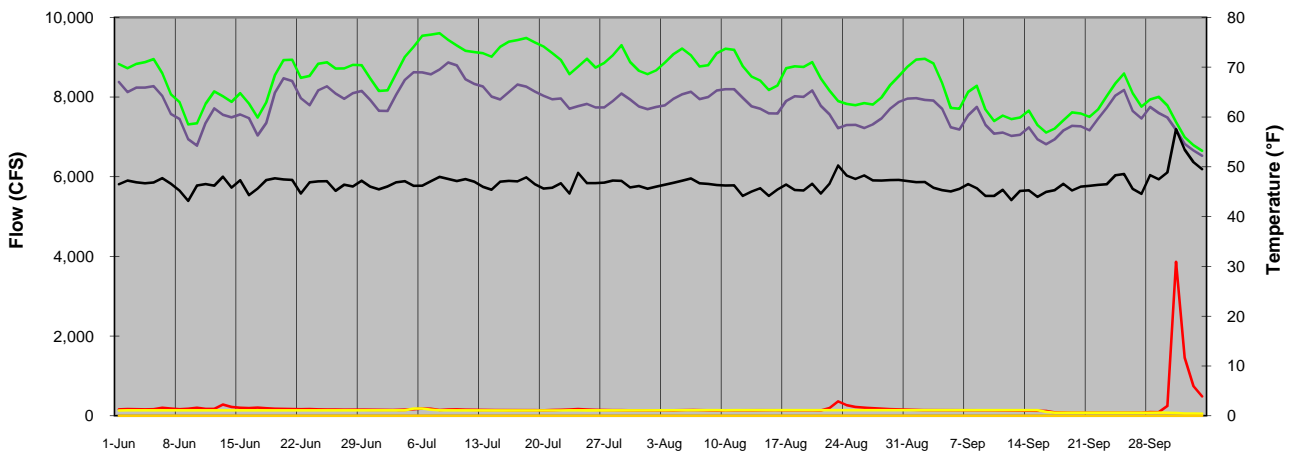
Figure 4: Longitudinal summer daily average water temperature profile on the East Branch at Downsville, Harvard, East Branch, and Fishes Eddy along with daily average flows at Downsville and Harvard, 2008-10.
