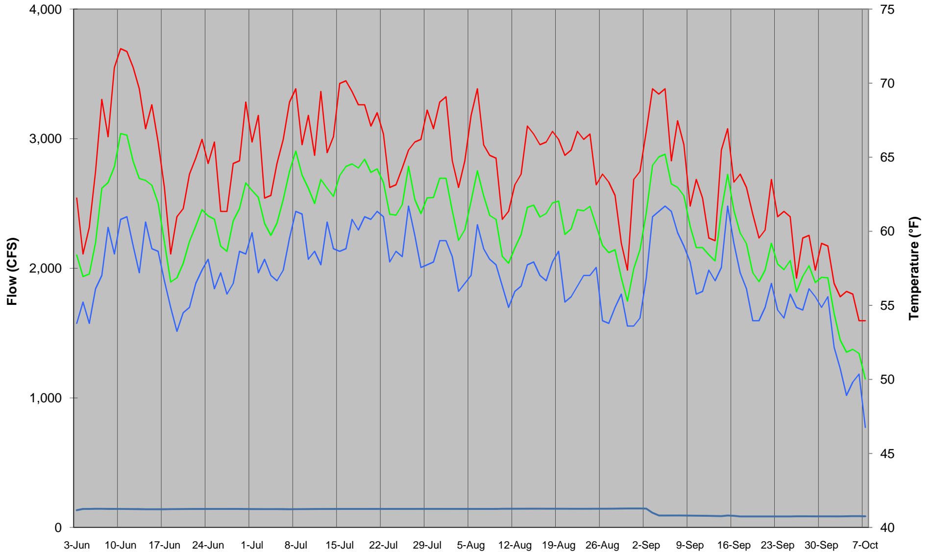
Appendix 1P. Summer daily average, maximum, and minimum water temperature profiles from the USGS gage on the East Branch at Harvard, along with daily average flows at Downsville, 2008.
