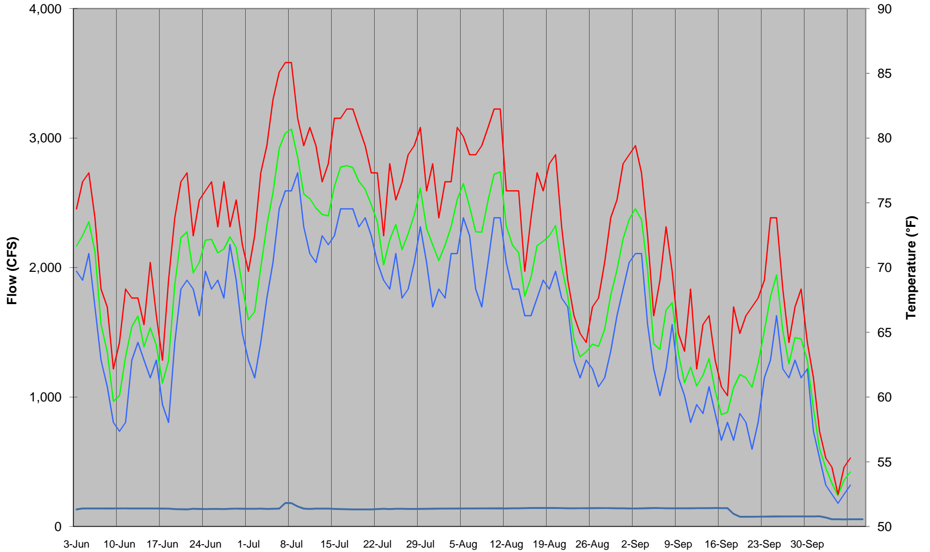
Appendix 3Q. Summer daily average, maximum, and minimum water temperature profiles on the East Branch at Hancock, along with daily average flows at Downsville, 2010.
