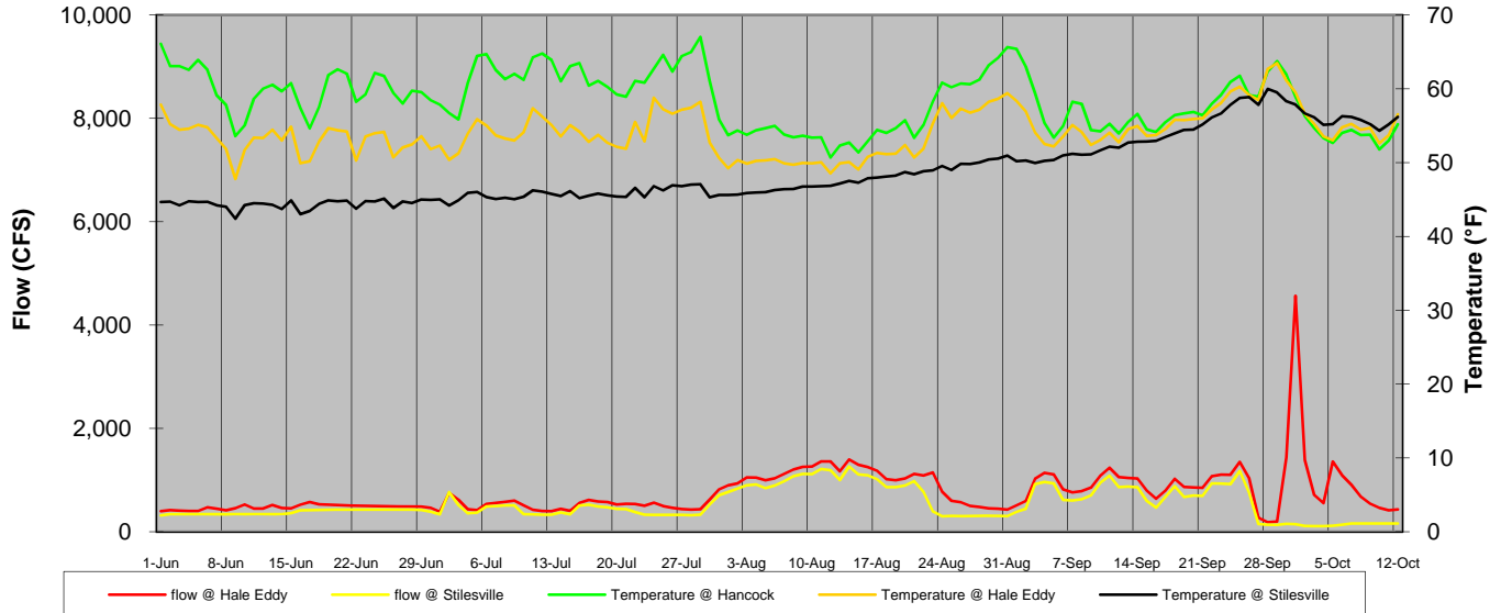
Figure 2: Longitudinal summer daily average water temperature profile on the West Branch at Stilesville, Hale Eddy, and Hancock along with daily average flows at Hale Eddy and Stilesville, 2008-2010.
