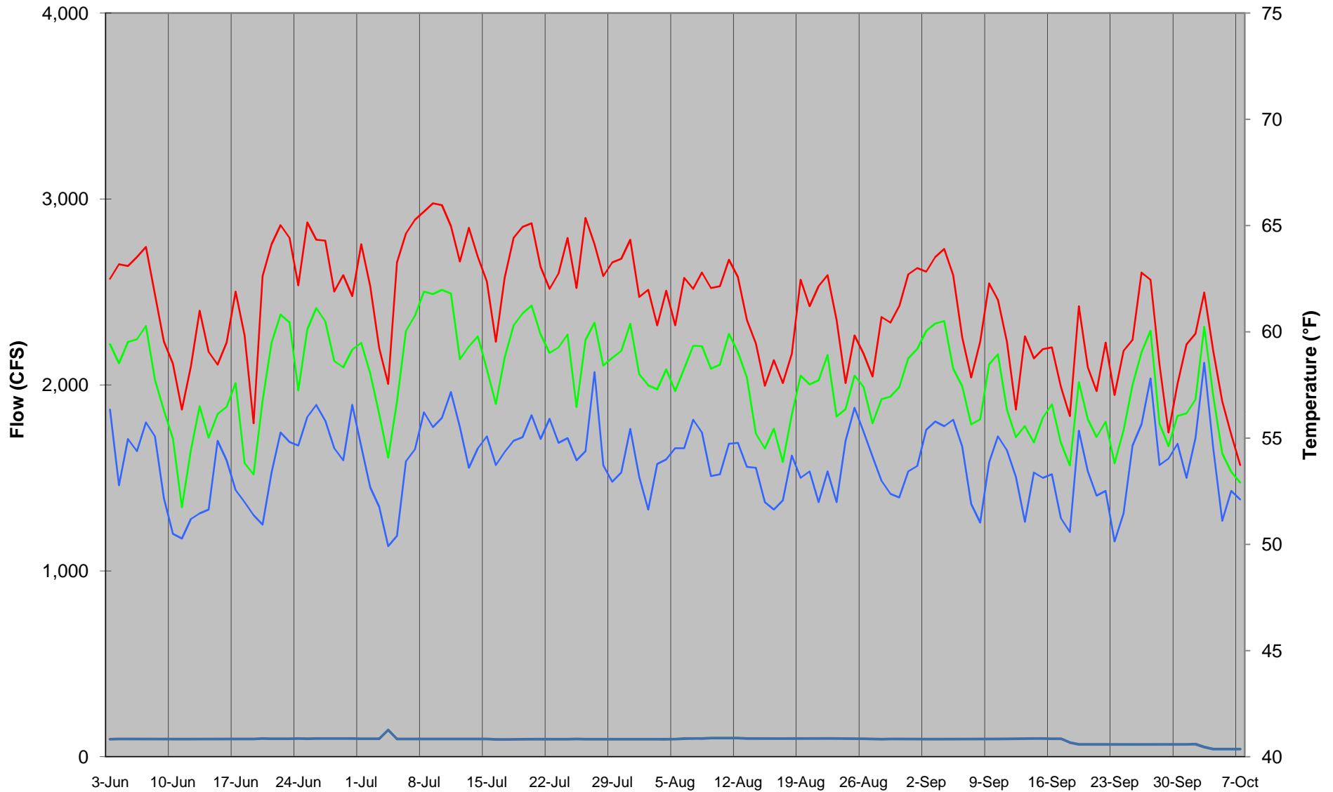
Appendix 3T. Summer daily average, maximum, and minimum water temperature profiles on the Neversink just above Fallsburg, along with daily average flows at Neversink, 2010.
